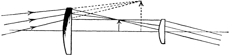
FIG. 59.—The Huyghenian Eye-piece.
