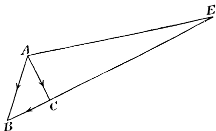
FIG. 89.—Proper Motion.
