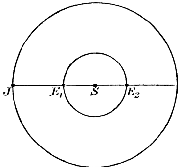
FIG. 82.—Roemer's Discovery.
