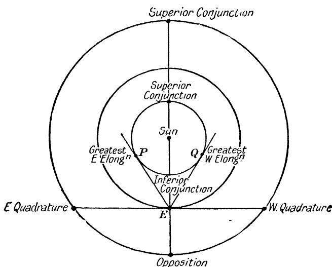
FIG. 75.—Planetary Configurations.
