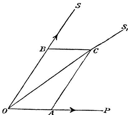
FIG. 27.—Aberration.
