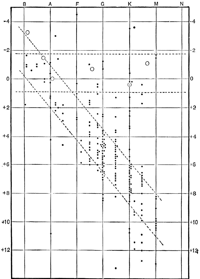
FIG. 95.—Giant and Dwarf Stars (Russell).
