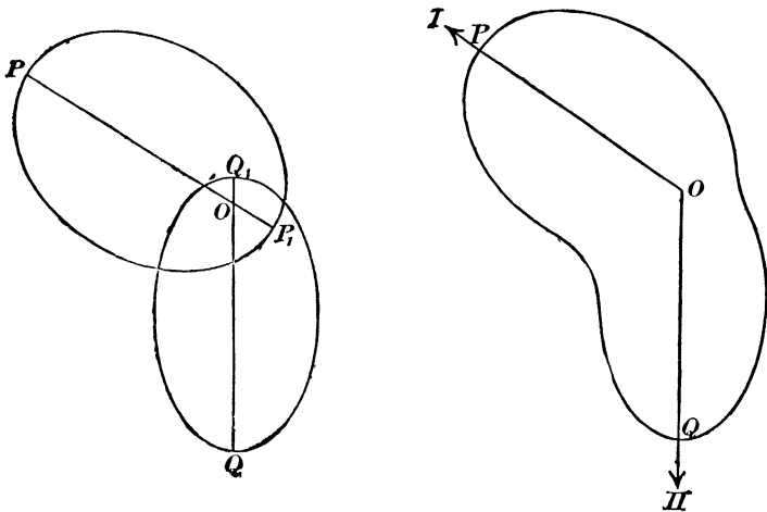
FIG. 92.—The Combination of two Single Drift Motions.
