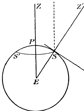
FIG. 73.—The Sub-Solar Point.
