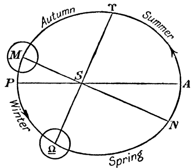
FIG. 16.—The Seasons.
