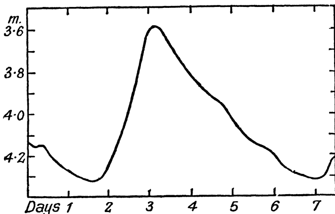
FIG. 98.—The Light Curve of \delta Cephei.
