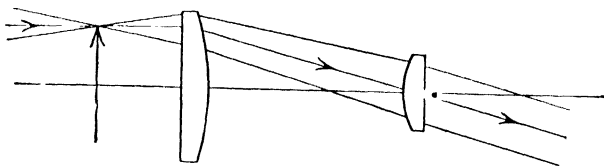
FIG. 58.—The Ramsden Eye-piece.
