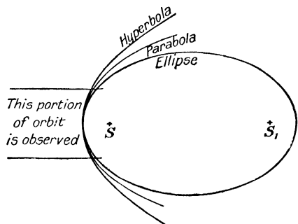
FIG. 84.—Cometary Orbits.
