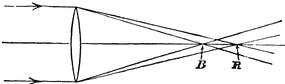
FIG. 56.—Chromatic Aberration.
