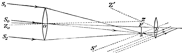
FIG. 53.—The Astronomical Refracting Telescope.
