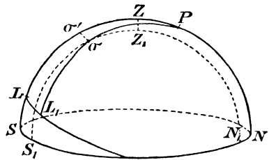
FIG. 65.—Collimation Error of Transit Instrument.
