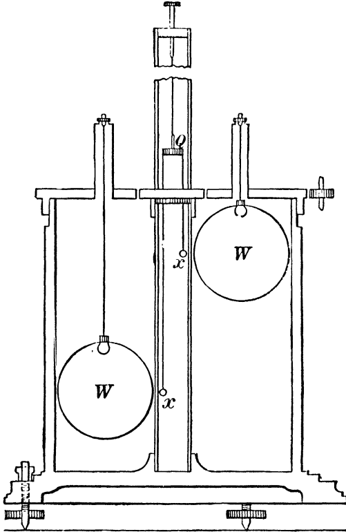
FIG. 8.—Boys' Torsion Balance.
