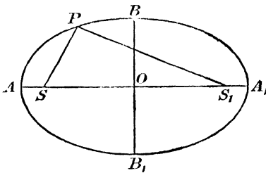
FIG. 14.—The Ellipse.
