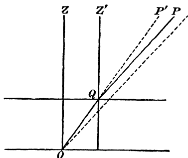
FIG. 11.—Elementary Theory of Refraction.
