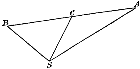
FIG. 93.—Star-streaming and Solar Motion.
