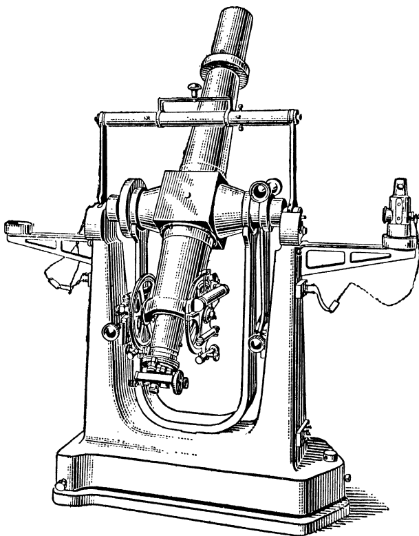
FIG. 61.—Three-inch Transit Instrument.
