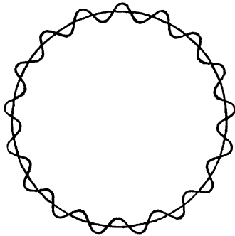
FIG. 26.—Nutation.
