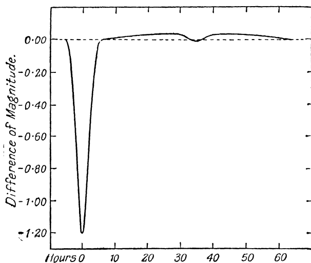
FIG. 101.—The Light Curve of Algol.
