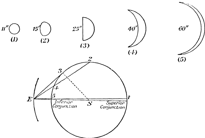
FIG. 80.—The Telescopic Appearances of Venus.
