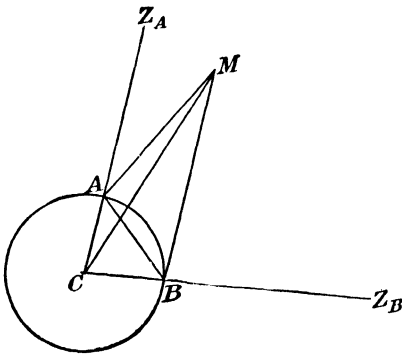
FIG. 37.—Determination of the Moon's Distance.
