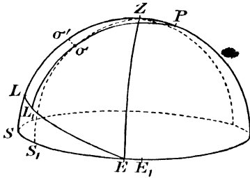
FIG. 64.—Azimuth Error of Transit Instrument.
