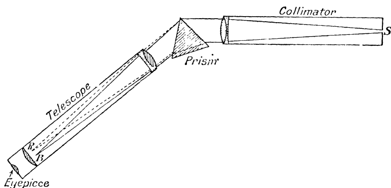
FIG. 69.—Diagram of Single Prism Spectroscope.
