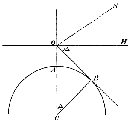
FIG. 12.—The Dip of the Horizon.
