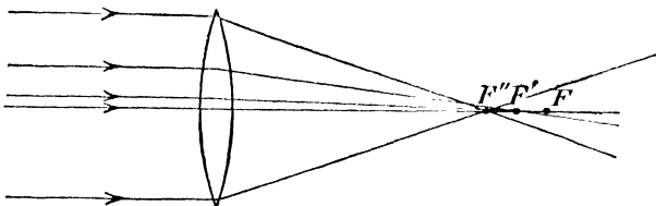
FIG. 55.—Spherical Aberration.
