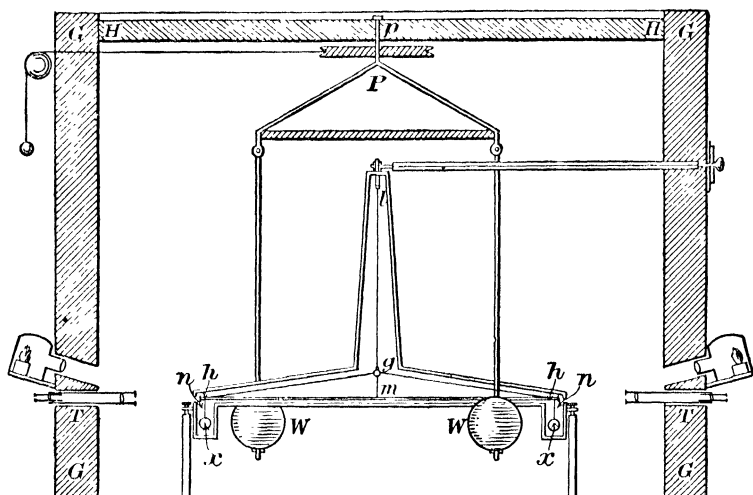
FIG. 7.—Cavendish's Apparatus.
