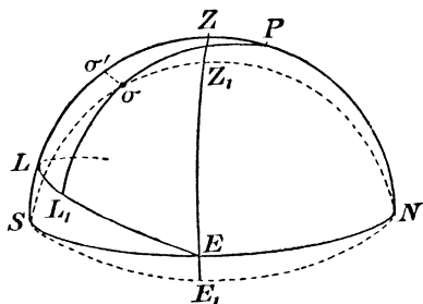
FIG. 63.—Level Error of Transit Instrument.
