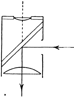
FIG. 62.—The Bohnenberger Eye-piece.
