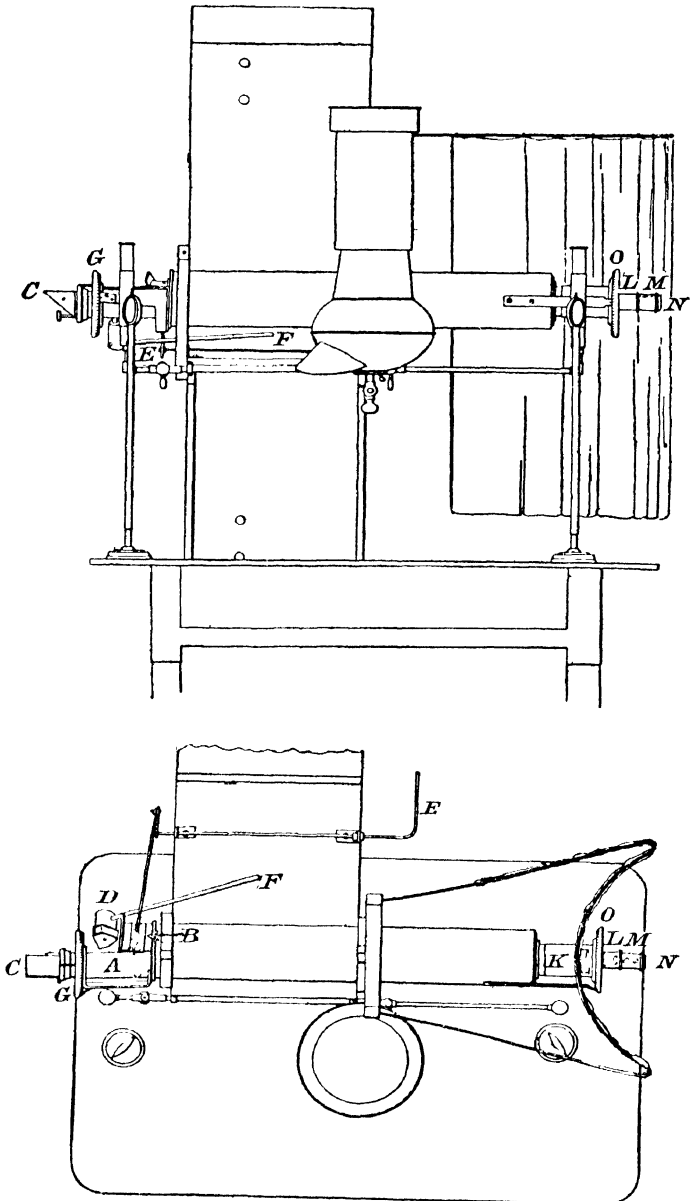
FIG. 88.—The Meridian Photometer.
