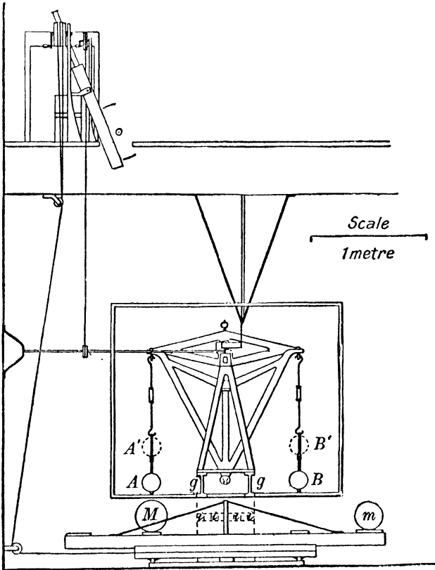
FIG. 9.—Poynting's Gravity Balance.
