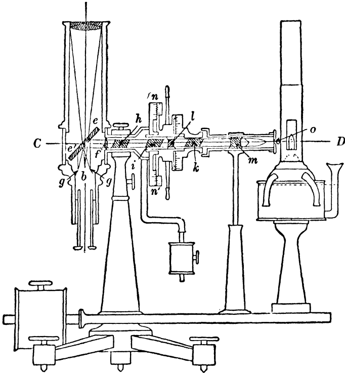
FIG. 87.—The Zöllner Photometer.
